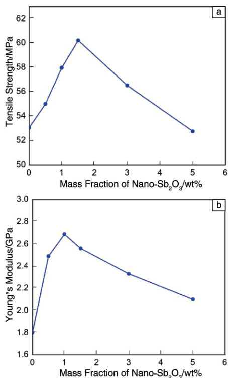
图 1 Nano-Sb 2 O 3 /BPS/PBT 复合材料的拉伸性能随 nano-Sb 2 O 3 含量变化的变化曲线: (a) 抗拉强度和 (b) 杨氏模量 Fig. 1 Variation curves of tensile properties of nano-Sb 2 O 3 /BPS/PBT composites with nano-Sb 2 O 3 contents: (a) tensile strength and (b) Young's modulus
