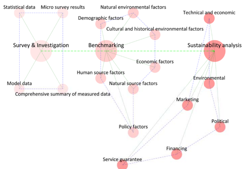
Figure 3. Methodological map.
